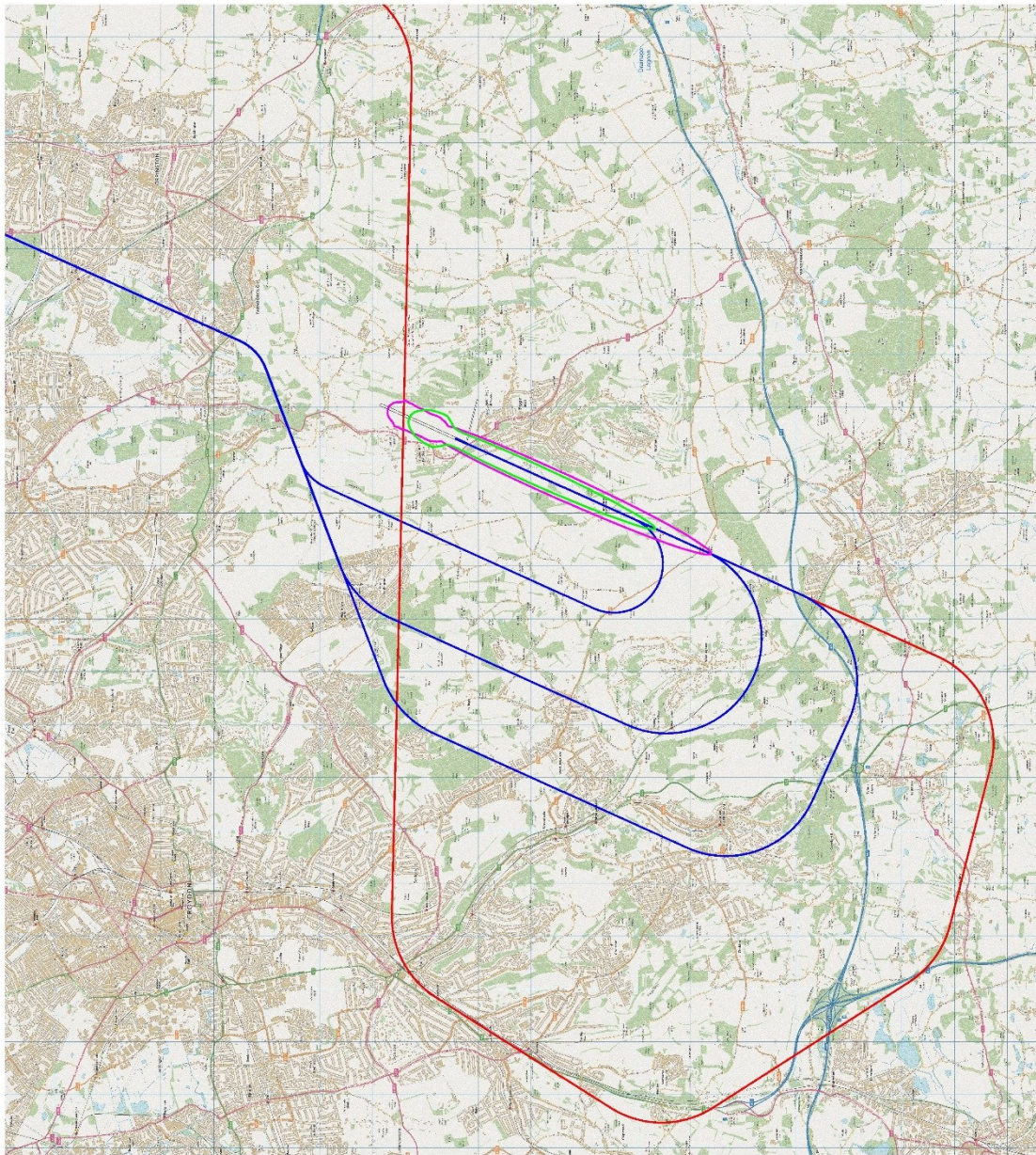
Figure 13: 80 dB(A) SEL Footprint (proposed Runway 03 RNAV GNSS arrival route)
