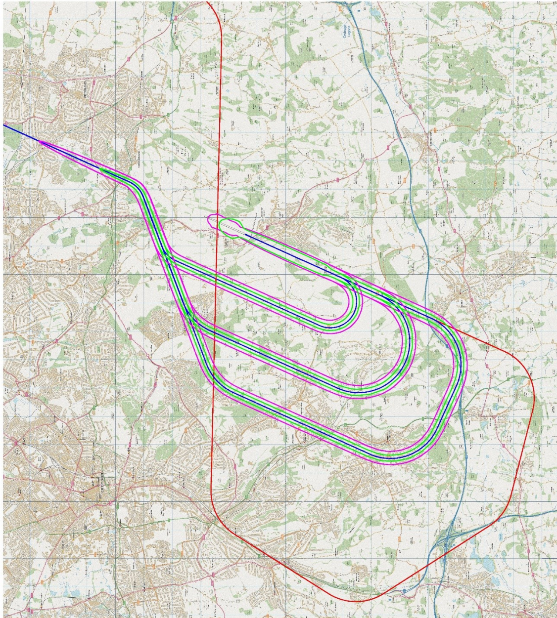
Figure 12: 80 dB(A) SEL Footprint (current Runway 03 arrival routes)
